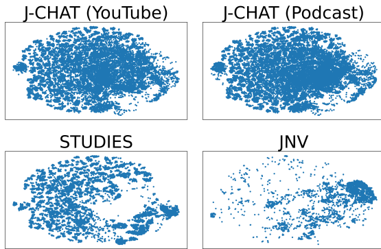
Fig. 2: Distribution of HuBERT [2] features extracted from J-CHAT (ours), STUDIES (simulated dialogue), and JNV (non-verbal expression).
